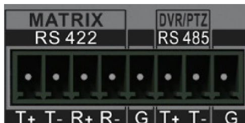
Figure 4-15 RS-485 Serial Port
